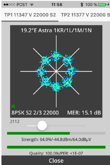
Figure 25: IQ measurement
